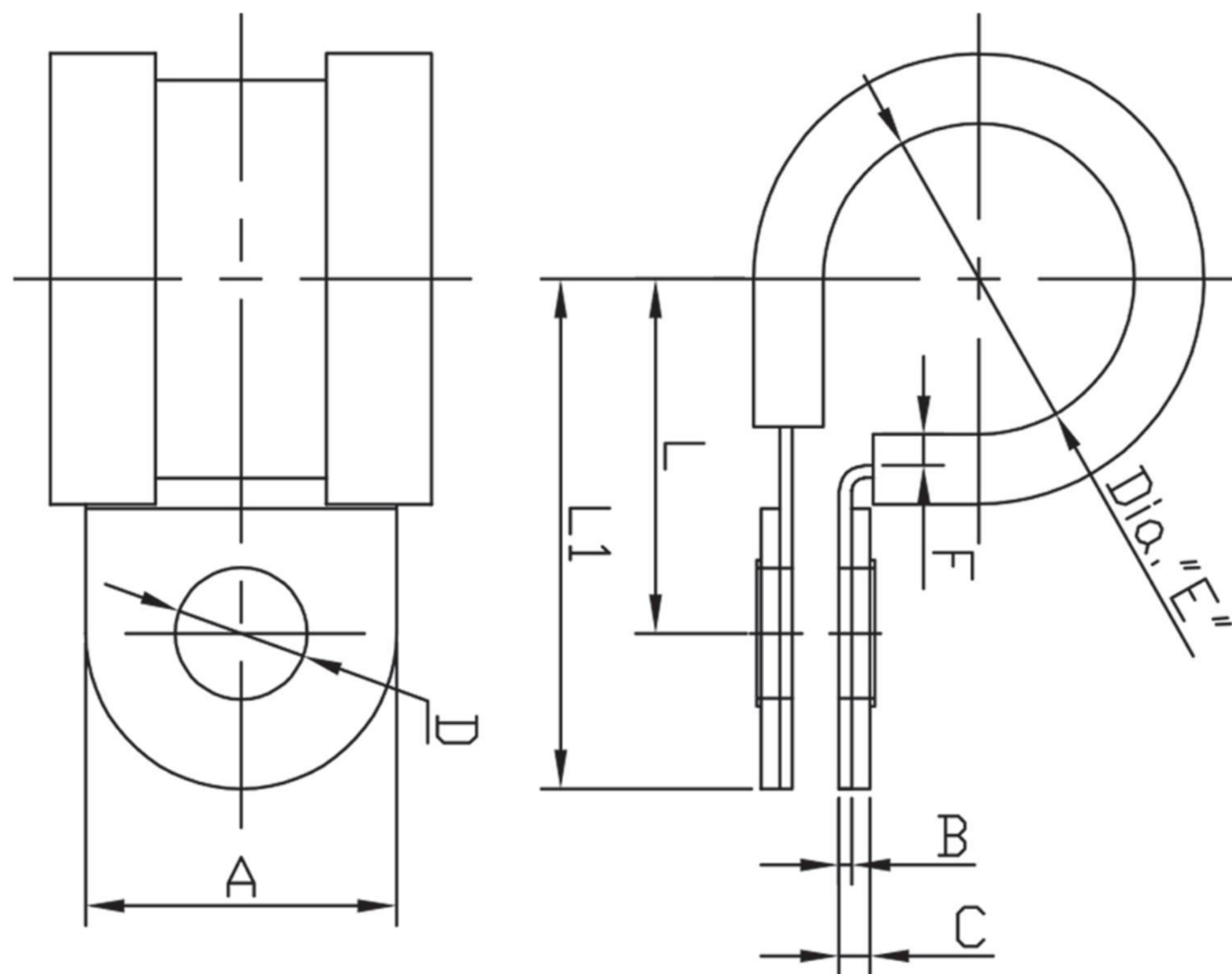
LJT01普通连胶条卡箍P-clip with rubber
